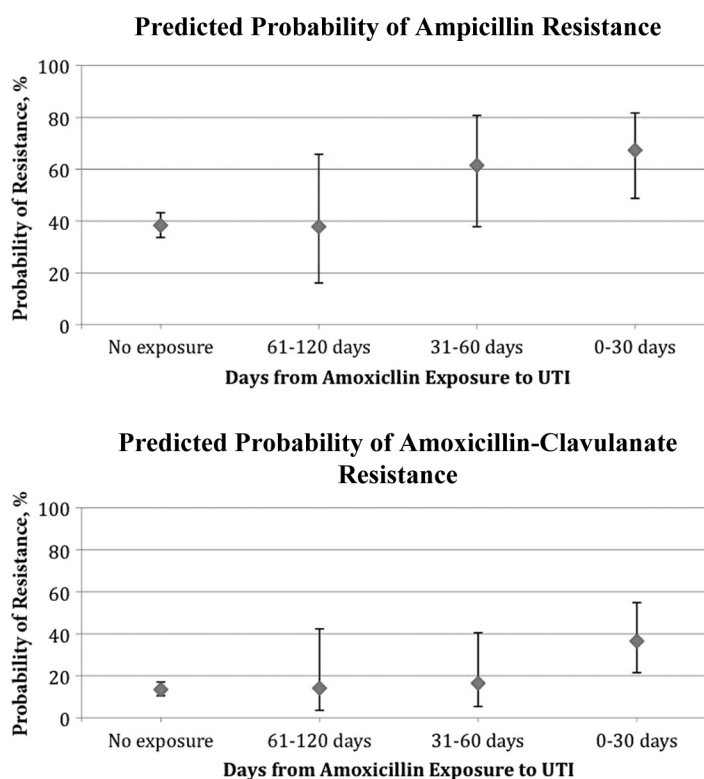
FIGURE 2 Predicted probability of resistance to ampicillin (top) and amoxicillin-clavulanate (bottom) given amoxicillin exposure within 120 days of UTI
