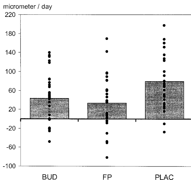
Fig 2. Mean (lines) and individual (circles) short-term lower-leg growth rates during treatment with BUD, FP, and Plac.
