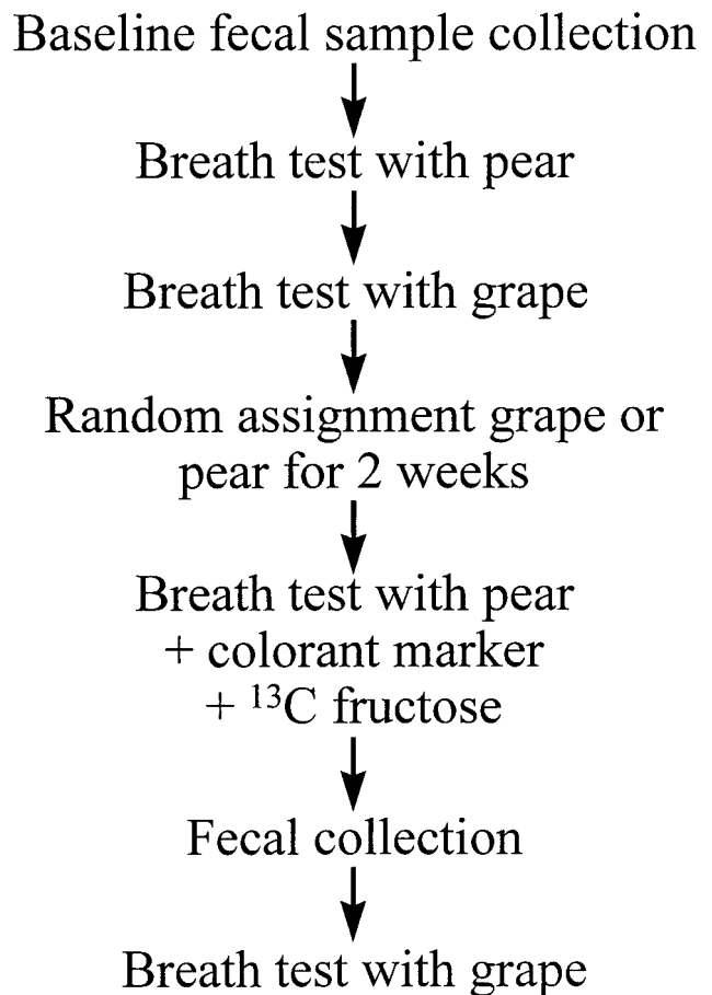
Fig 1. Protocol design.
